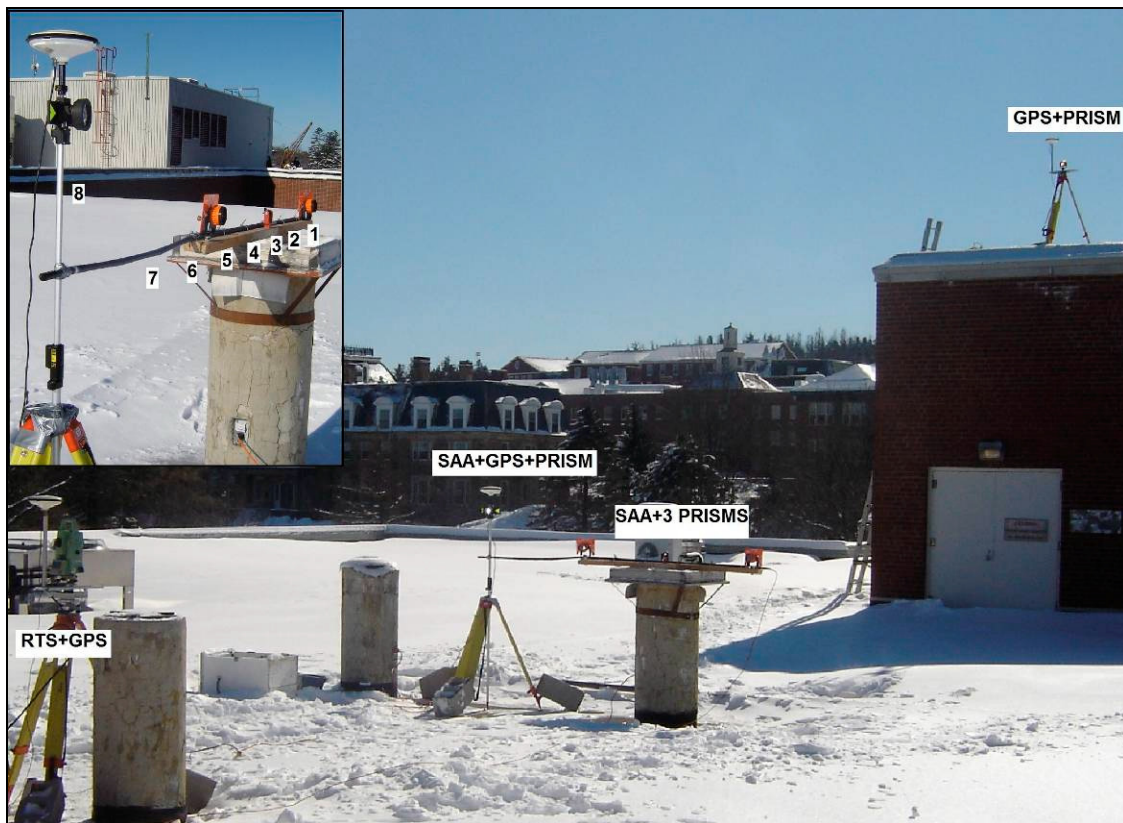
Figure 4: Integrated Technology Solution for Deformation Monitoring Scenario
