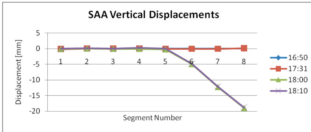
Figure 5: SAA Vertical Displacements
