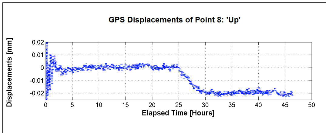
Figure 6: Up Component Displacement of Point 8 from PPM
